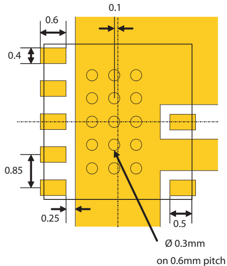
Figure 15. Metallization
