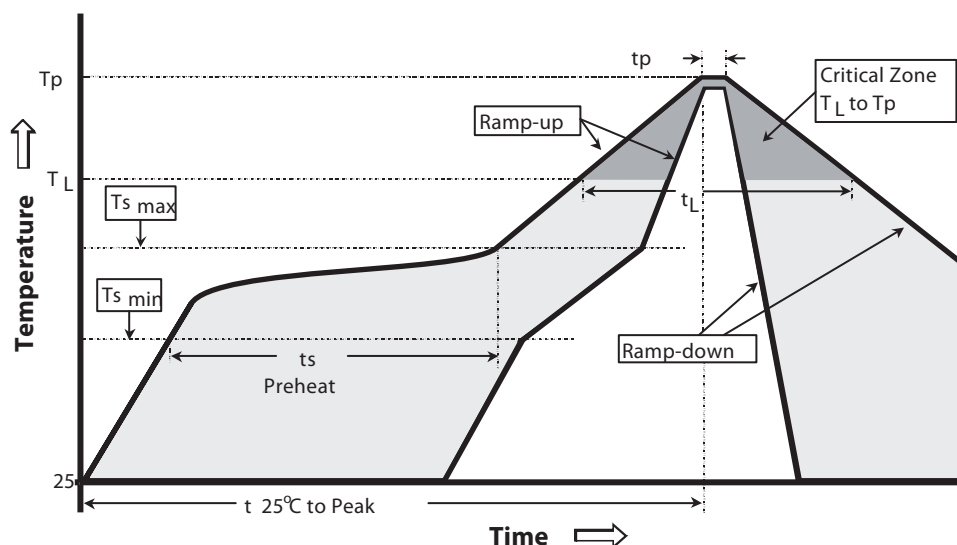
Figure 20. Typical SMT Reflow Profile for Maximum Temperature = 260 \pm 5^\circ\text{C}
